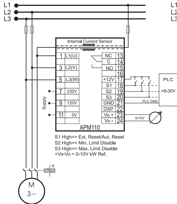
Fig.4 Typical connection with internal sensor
